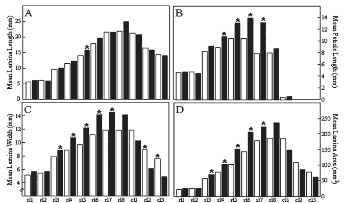
Fig. 2. Mean of the lamina length (A), petiole length (B), lamina width (C), and lamina area (D) of eight rosette leaves (r11 to r18) and three cauline leaves (c11 to c13) ( n=15 ), of 5-week-old ron2-1 mutant (black bars) and wild-type ( Ler ) plants (white bars). The asterisks indicate a statistically significant difference between mutant and wild type ( t -test, P < 0.05 ).
